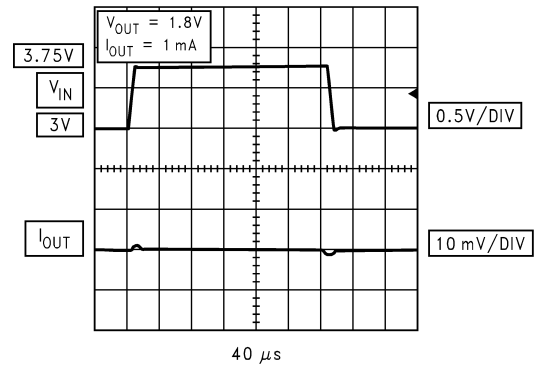
LDO Line Transient Response
